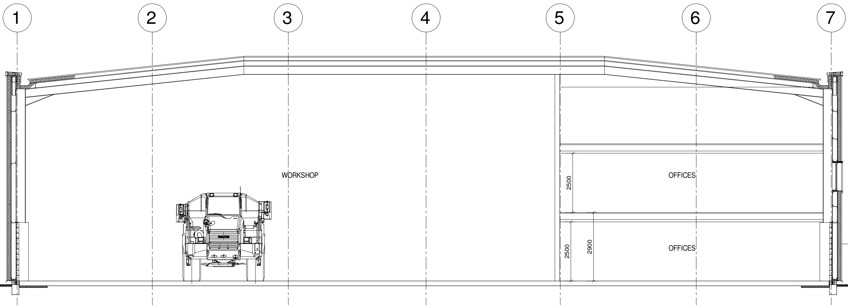
PROPOSED SECTION B - B
